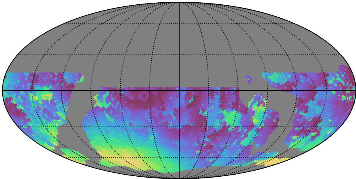
weather_cloudso6v3.4_10yrs WFD u band: Min moonDistance
