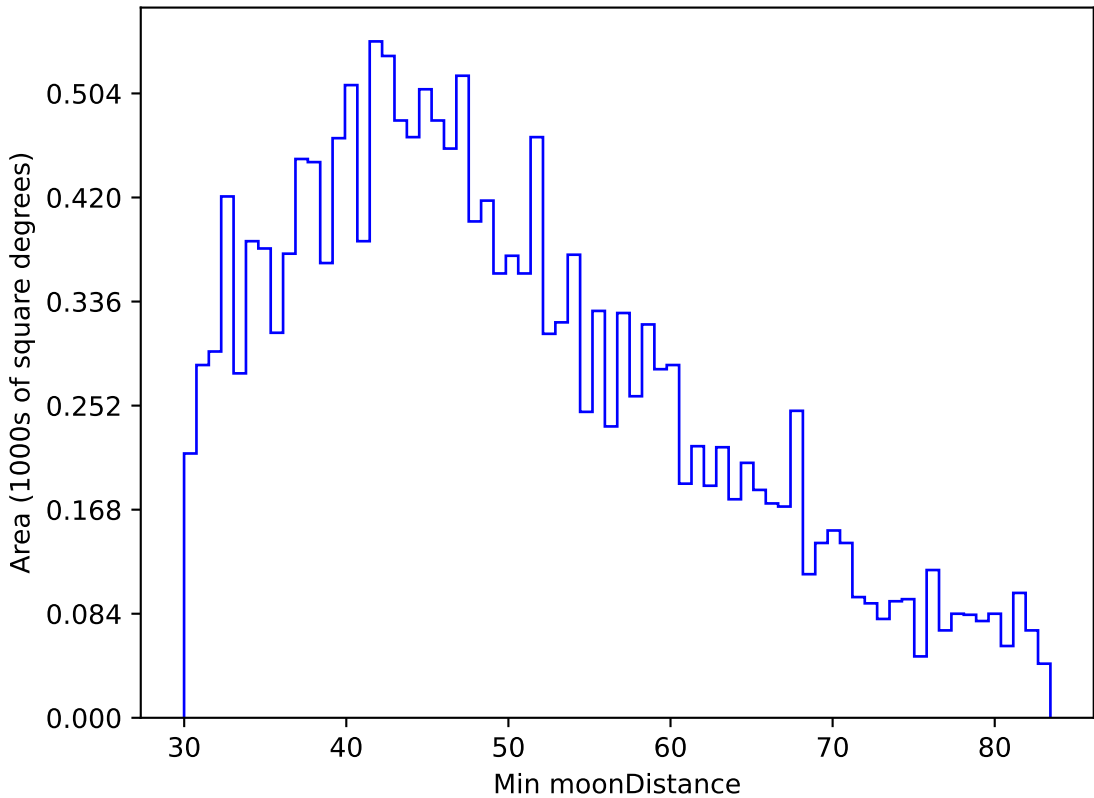
weather_cloudso6v3.4_10yrs WFD u band: Min moonDistance
