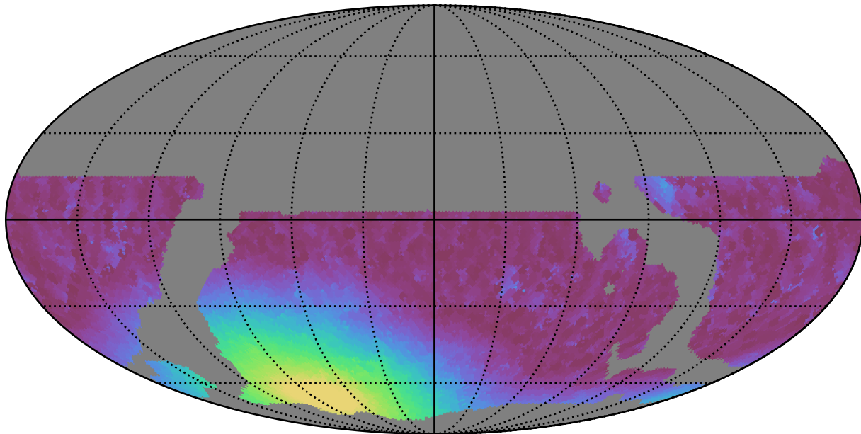
weather_cloudso6v3.4_10yrs WFD r band: Min moonDistance
