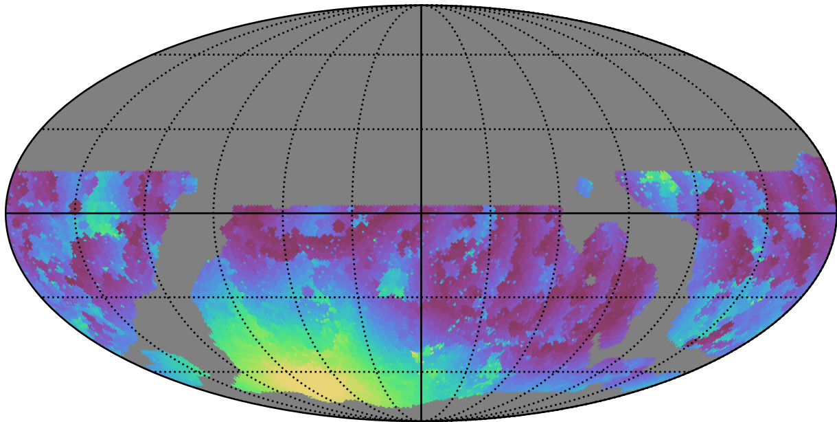
weather_cloudso6v3.4_10yrs WFD g band: Min moonDistance
