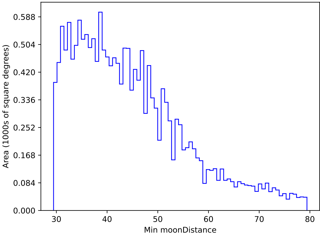
weather_cloudso6v3.4_10yrs WFD g band: Min moonDistance
