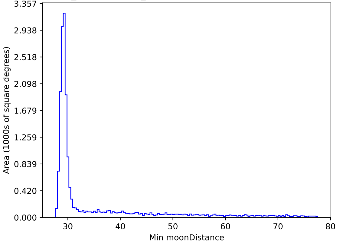
weather_cloudso6v3.4_10yrs WFD all bands: Min moonDistance
