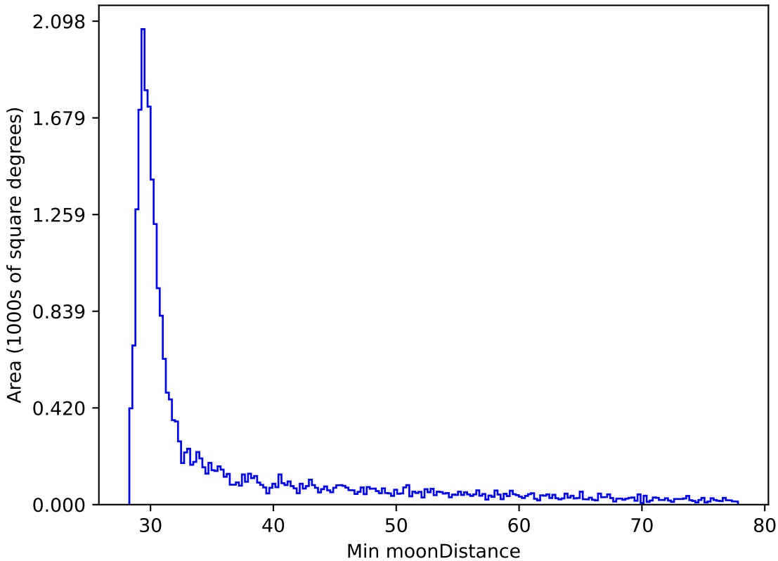
weather_cloudso6v3.4_10yrs All sky z band: Min moonDistance
