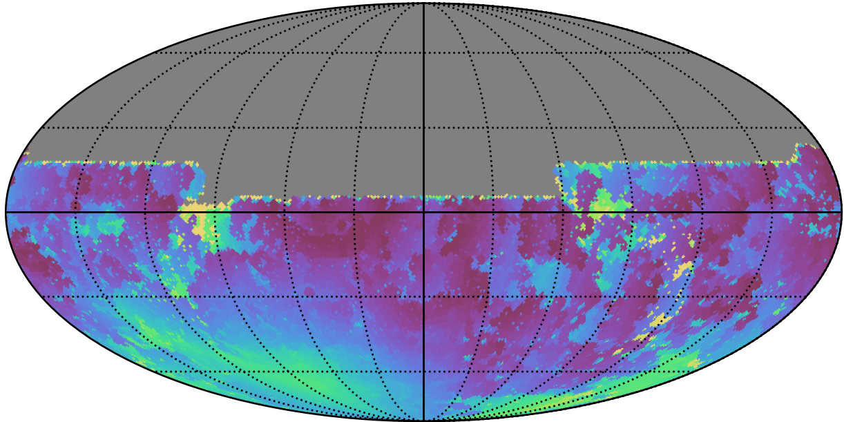
weather_cloudso6v3.4_10yrs All sky u band: Min moonDistance
