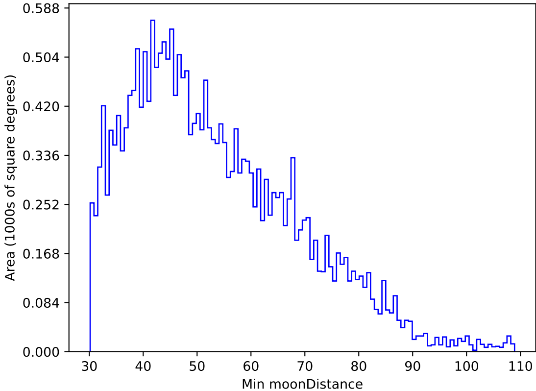
weather_cloudso6v3.4_10yrs All sky u band: Min moonDistance
