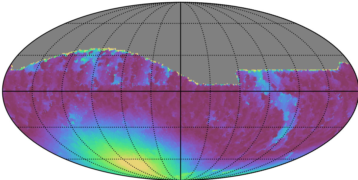
weather_cloudso6v3.4_10yrs All sky r band: Min moonDistance
