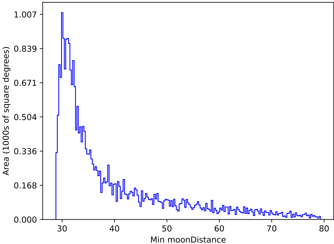
weather_cloudso6v3.4_10yrs All sky r band: Min moonDistance
