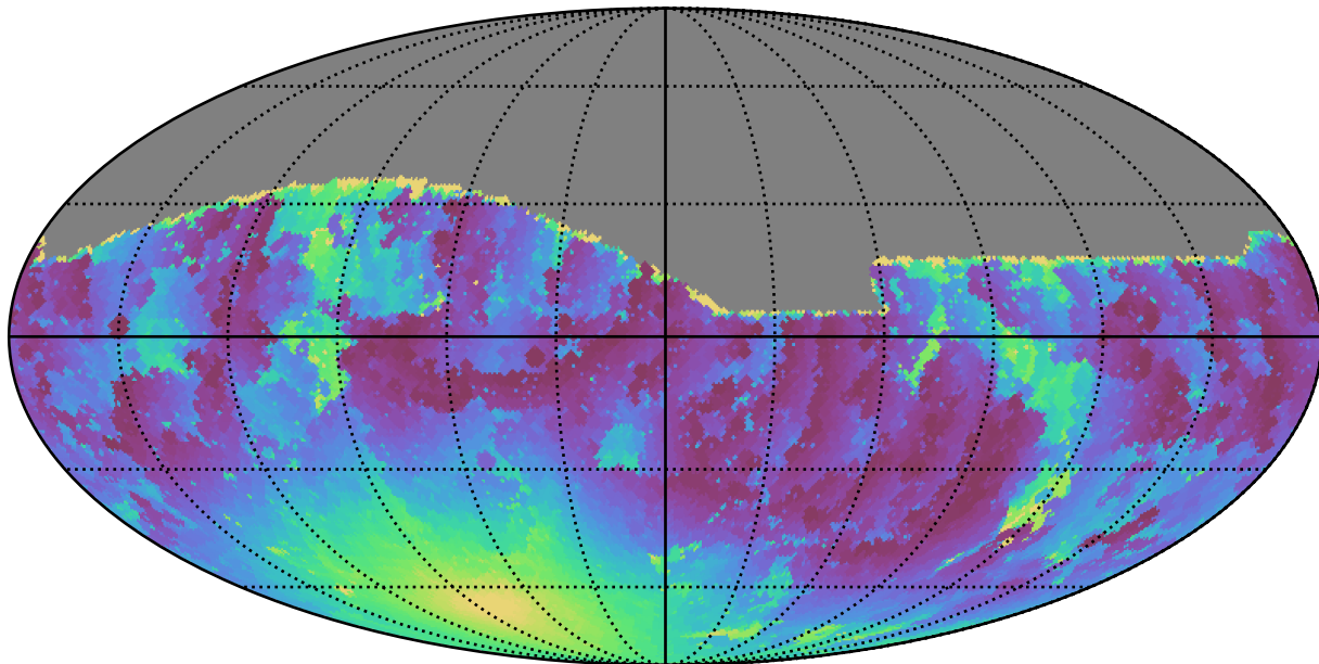
weather_cloudso6v3.4_10yrs All sky g band: Min moonDistance
