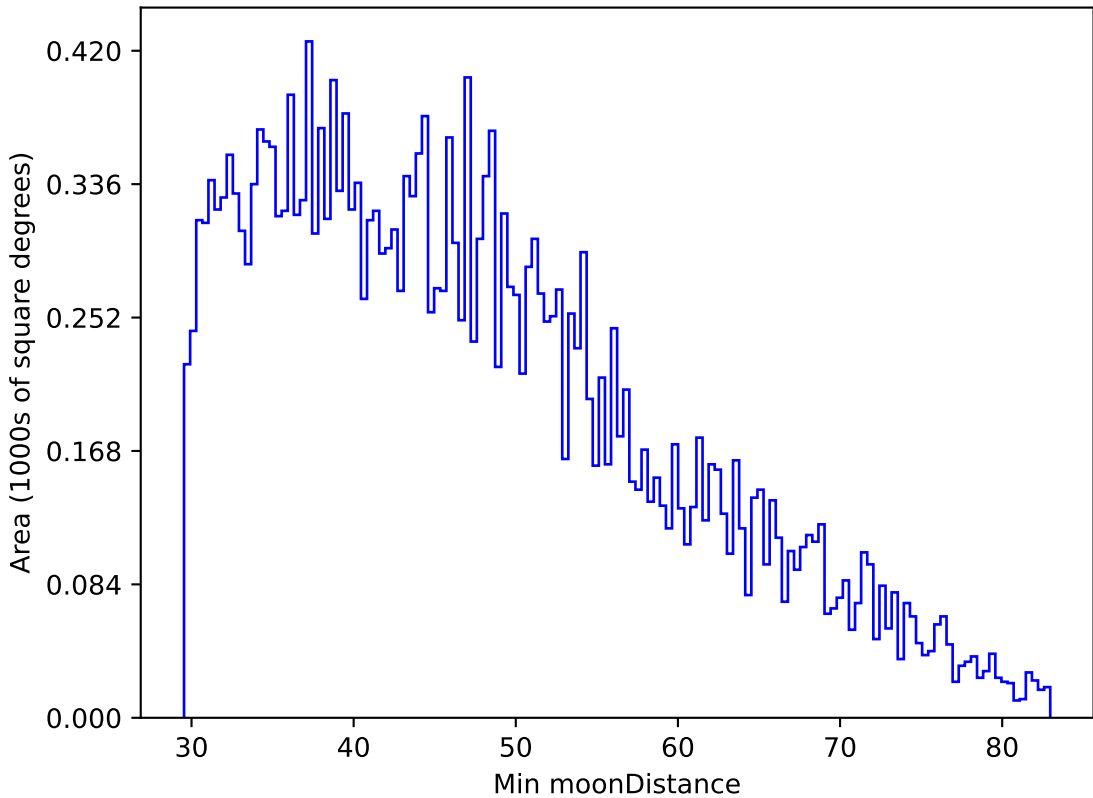
weather_cloudso6v3.4_10yrs All sky g band: Min moonDistance
