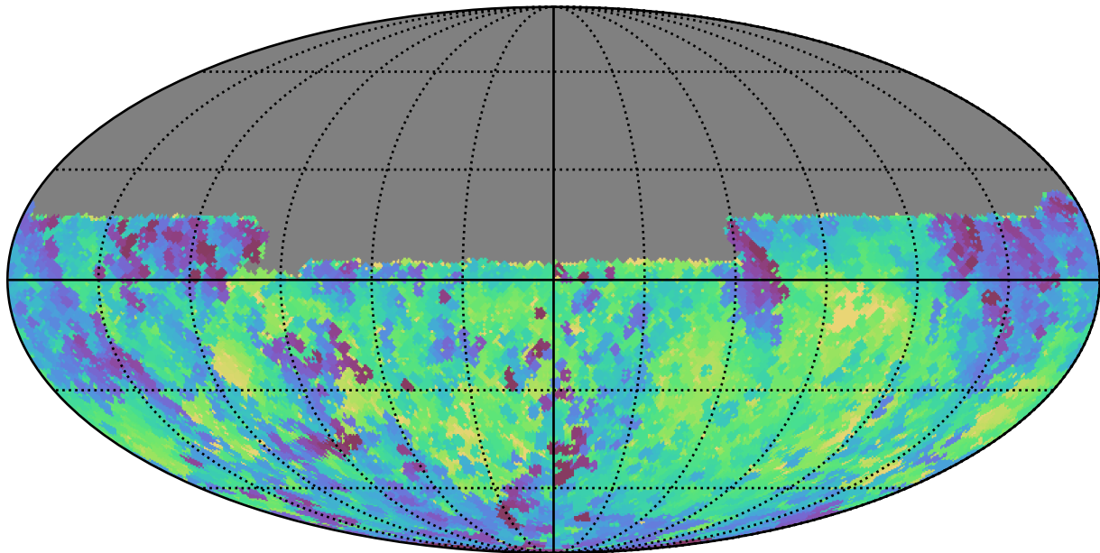
weather_cloudso6v3.4_10yrs Yr 1 y band: Min fiveSigmaDepth
