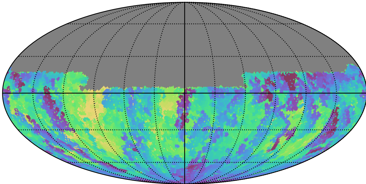
weather_cloudso6v3.4_10yrs Yr 1 u band: Min fiveSigmaDepth
