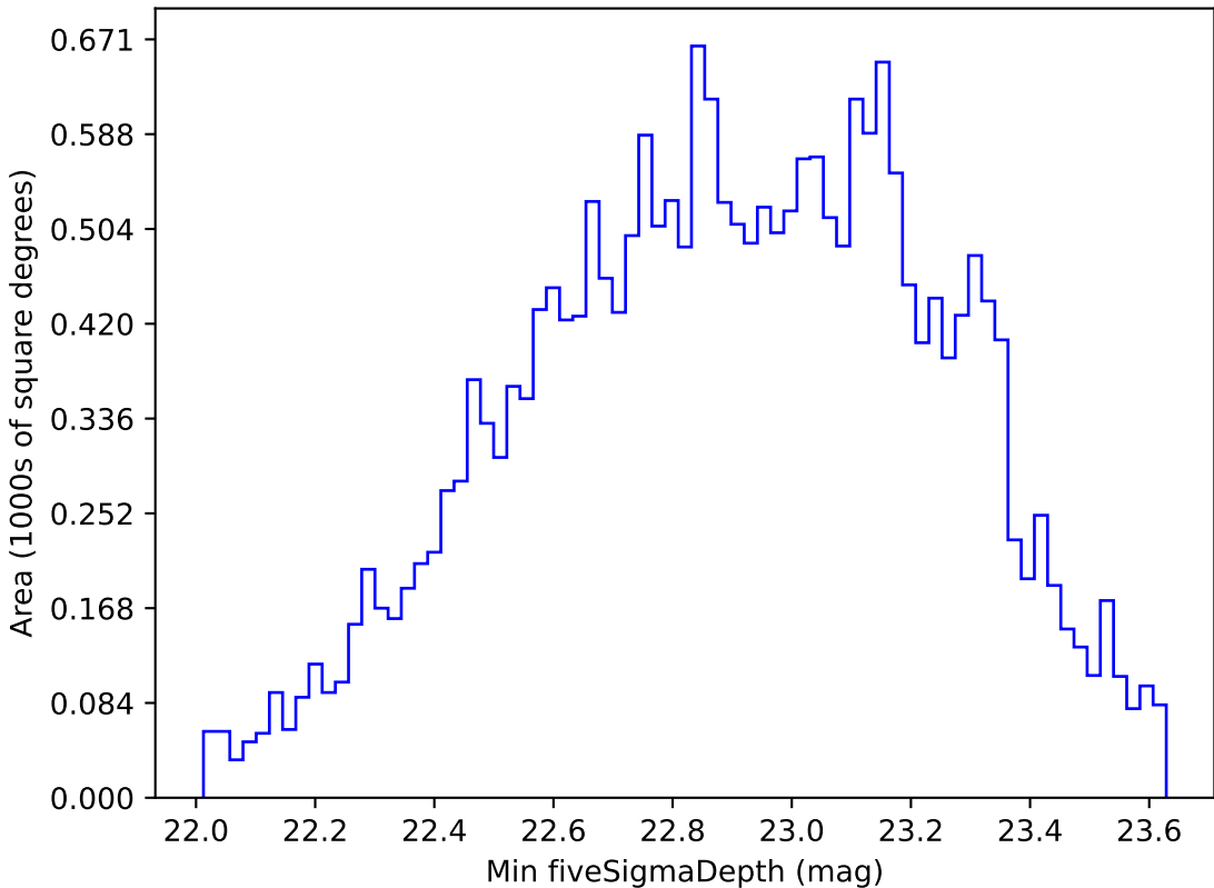
weather_cloudso6v3.4_10yrs Yr 1 u band: Min fiveSigmaDepth
