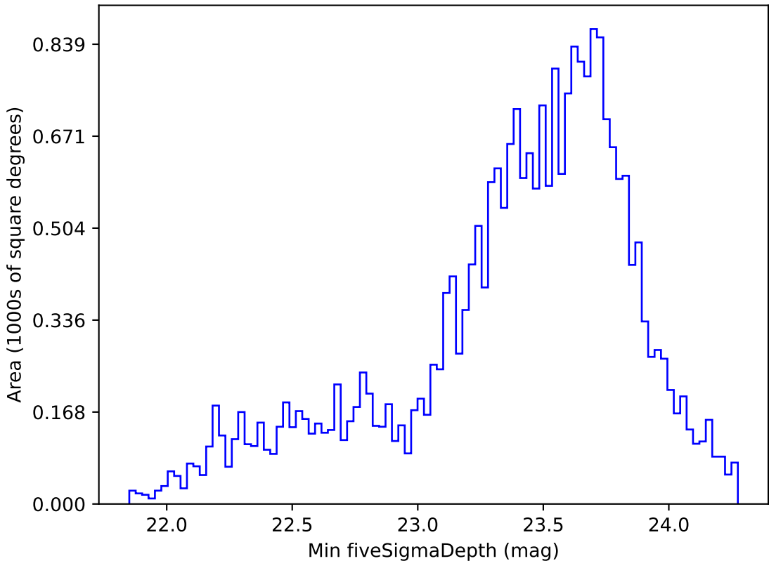
weather_cloudso6v3.4_10yrs Yr 1 r band: Min fiveSigmaDepth
