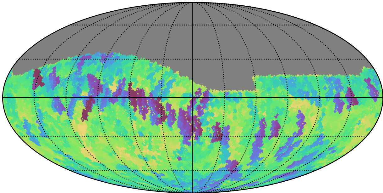
weather_cloudso6v3.4_10yrs Yr 1 i band: Min fiveSigmaDepth
