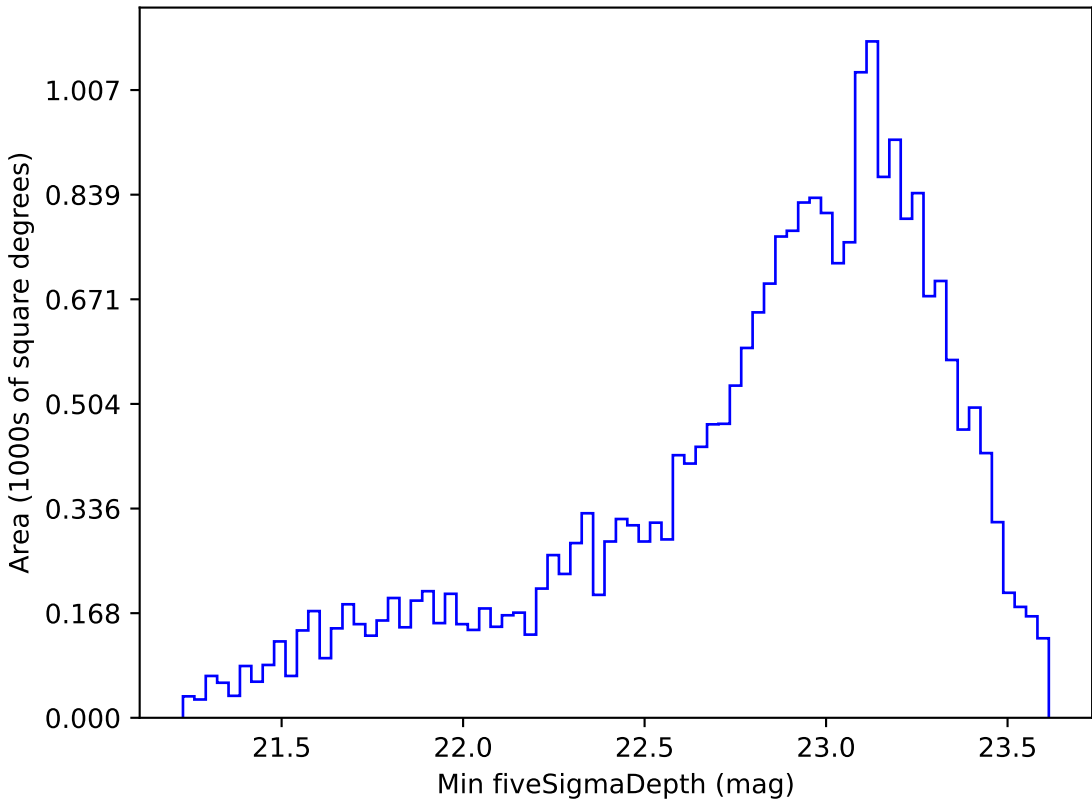
weather_cloudso6v3.4_10yrs Yr 1 i band: Min fiveSigmaDepth
