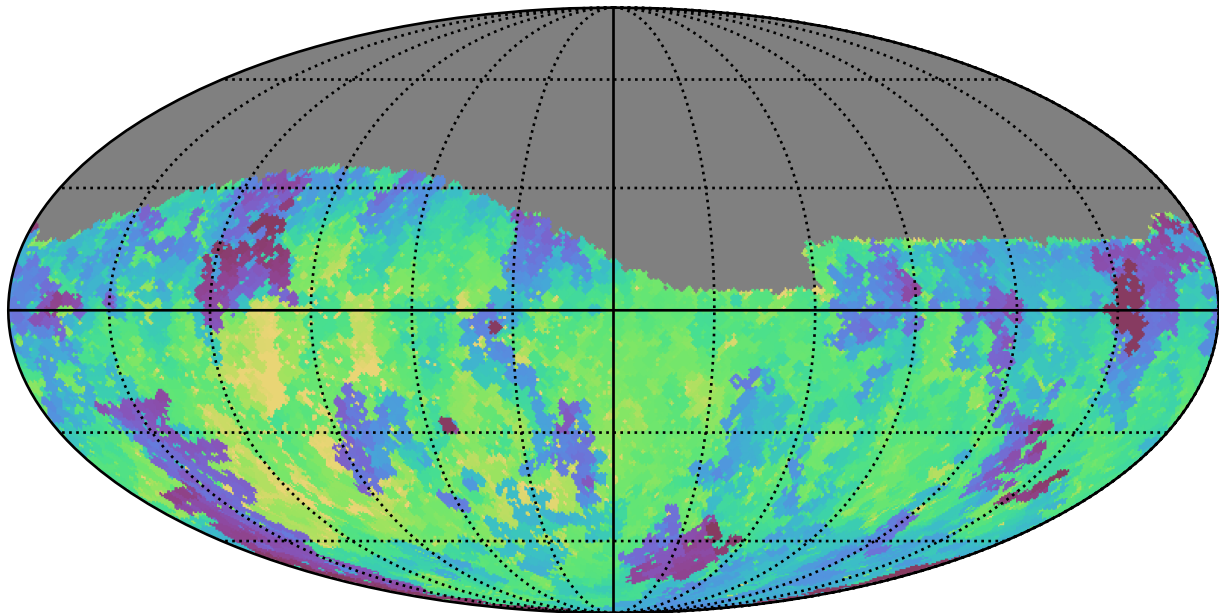
weather_cloudso6v3.4_10yrs Yr 1 g band: Min fiveSigmaDepth
