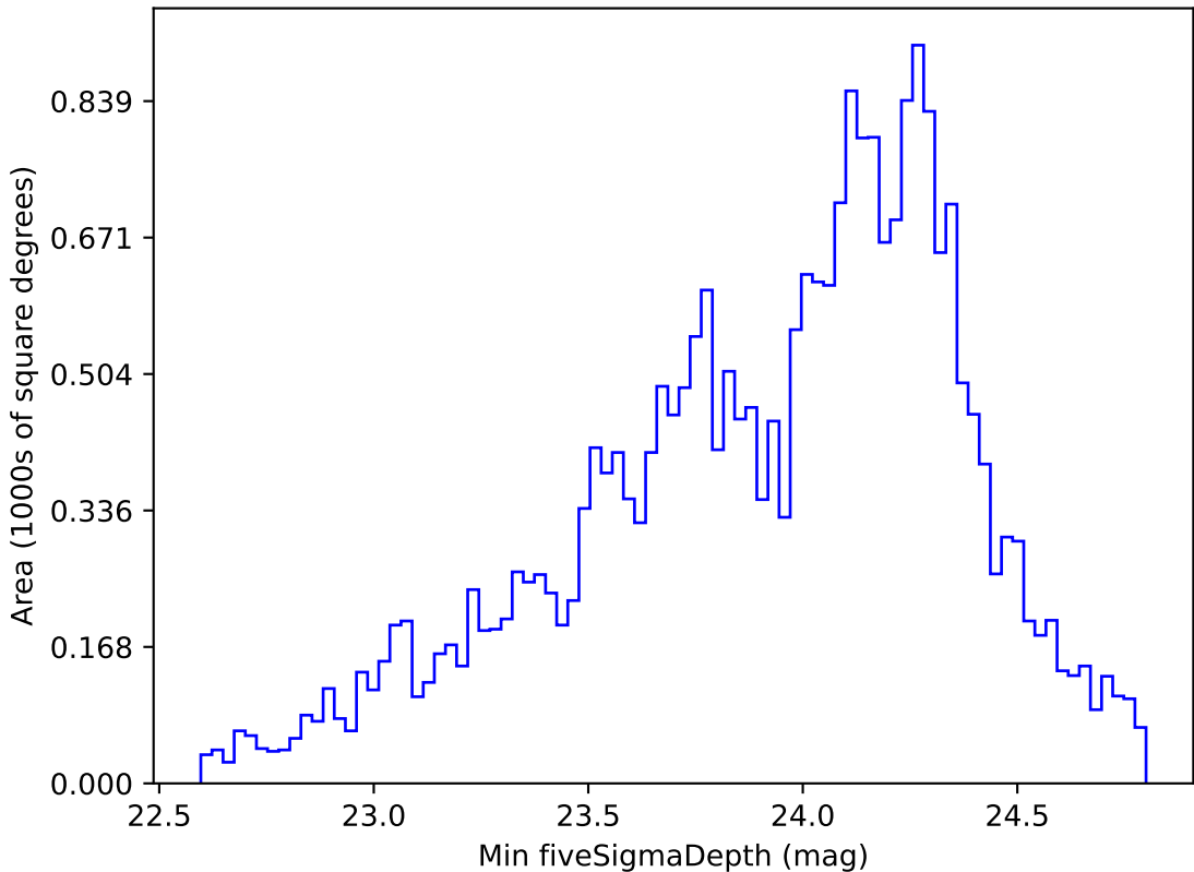
weather_cloudso6v3.4_10yrs Yr 1 g band: Min fiveSigmaDepth
