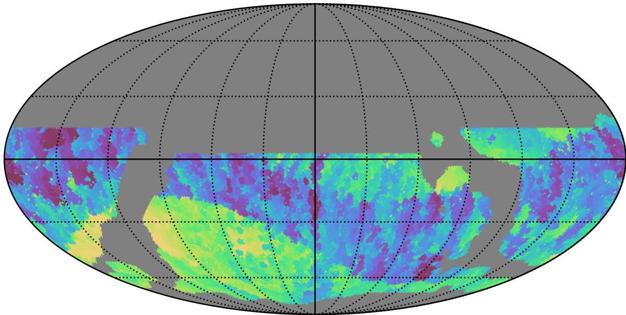
weather_cloudso6v3.4_10yrs WFD z band: Min fiveSigmaDepth
