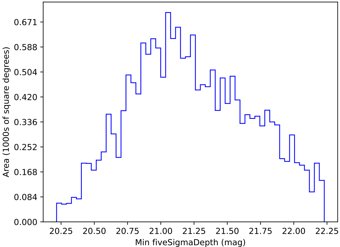
weather_cloudso6v3.4_10yrs WFD z band: Min fiveSigmaDepth
