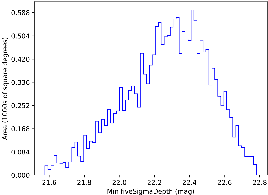
weather_cloudso6v3.4_10yrs WFD u band: Min fiveSigmaDepth
