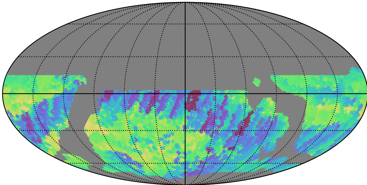
weather_cloudso6v3.4_10yrs WFD r band: Min fiveSigmaDepth
