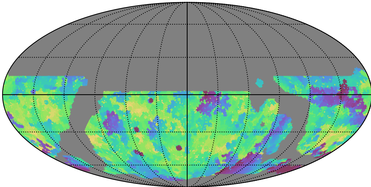
weather_cloudso6v3.4_10yrs WFD g band: Min fiveSigmaDepth
