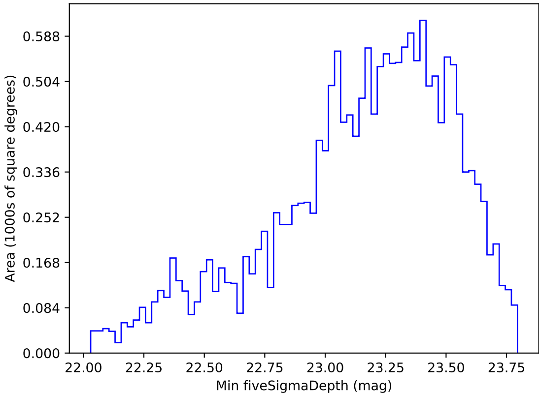
weather_cloudso6v3.4_10yrs WFD g band: Min fiveSigmaDepth
