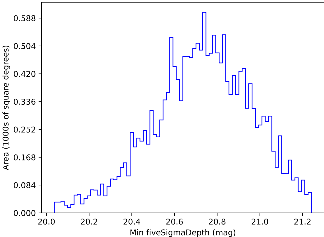
weather_cloudso6v3.4_10yrs WFD all bands: Min fiveSigmaDepth
