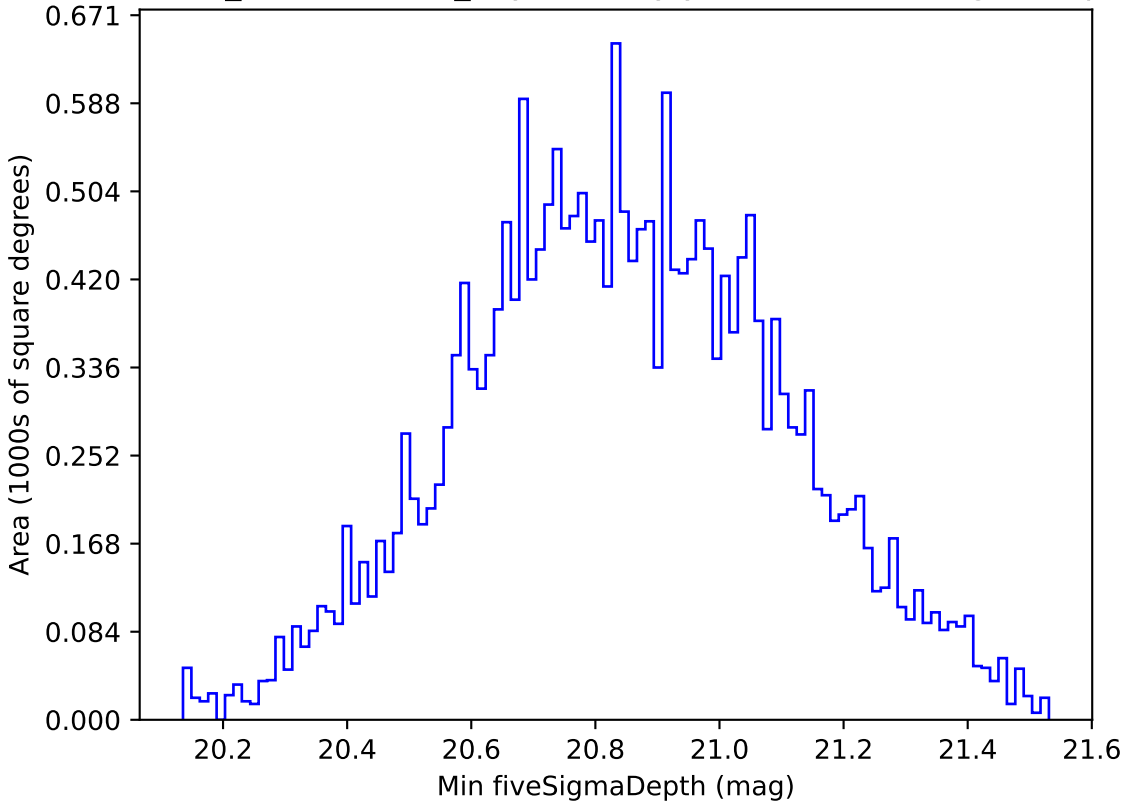
weather_cloudso6v3.4_10yrs All sky y band: Min fiveSigmaDepth
