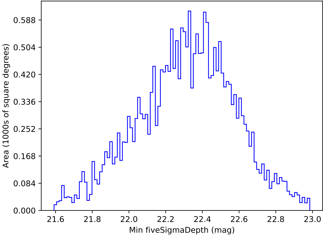
weather_cloudso6v3.4_10yrs All sky u band: Min fiveSigmaDepth
