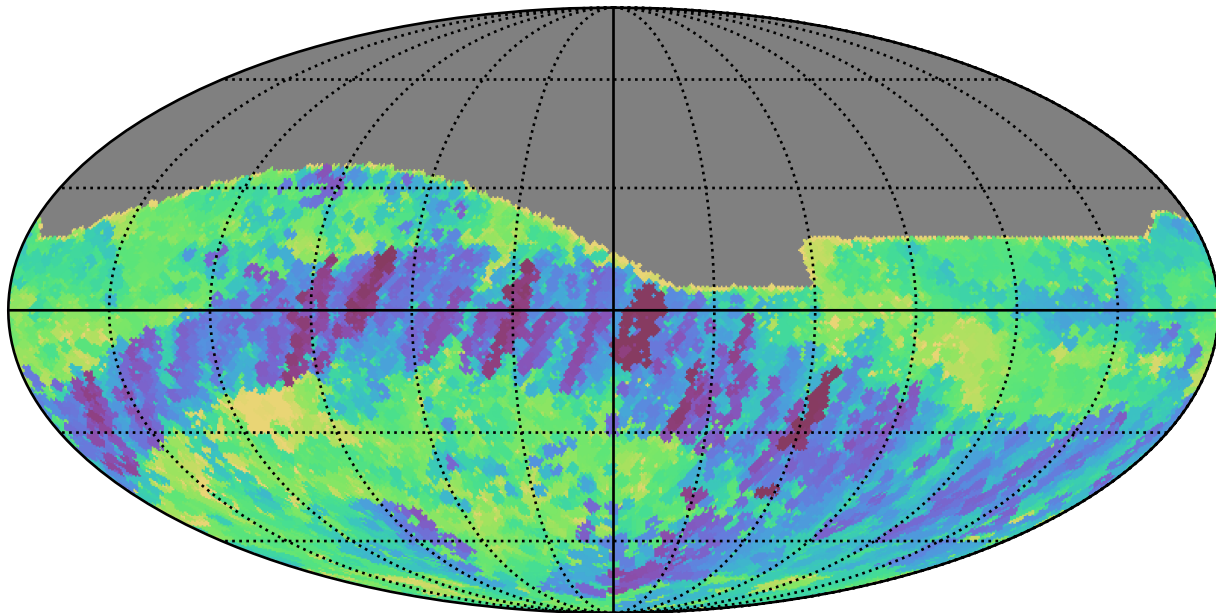
weather_cloudso6v3.4_10yrs All sky r band: Min fiveSigmaDepth
