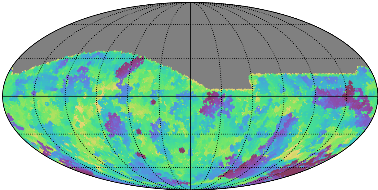
weather_cloudso6v3.4_10yrs All sky g band: Min fiveSigmaDepth
