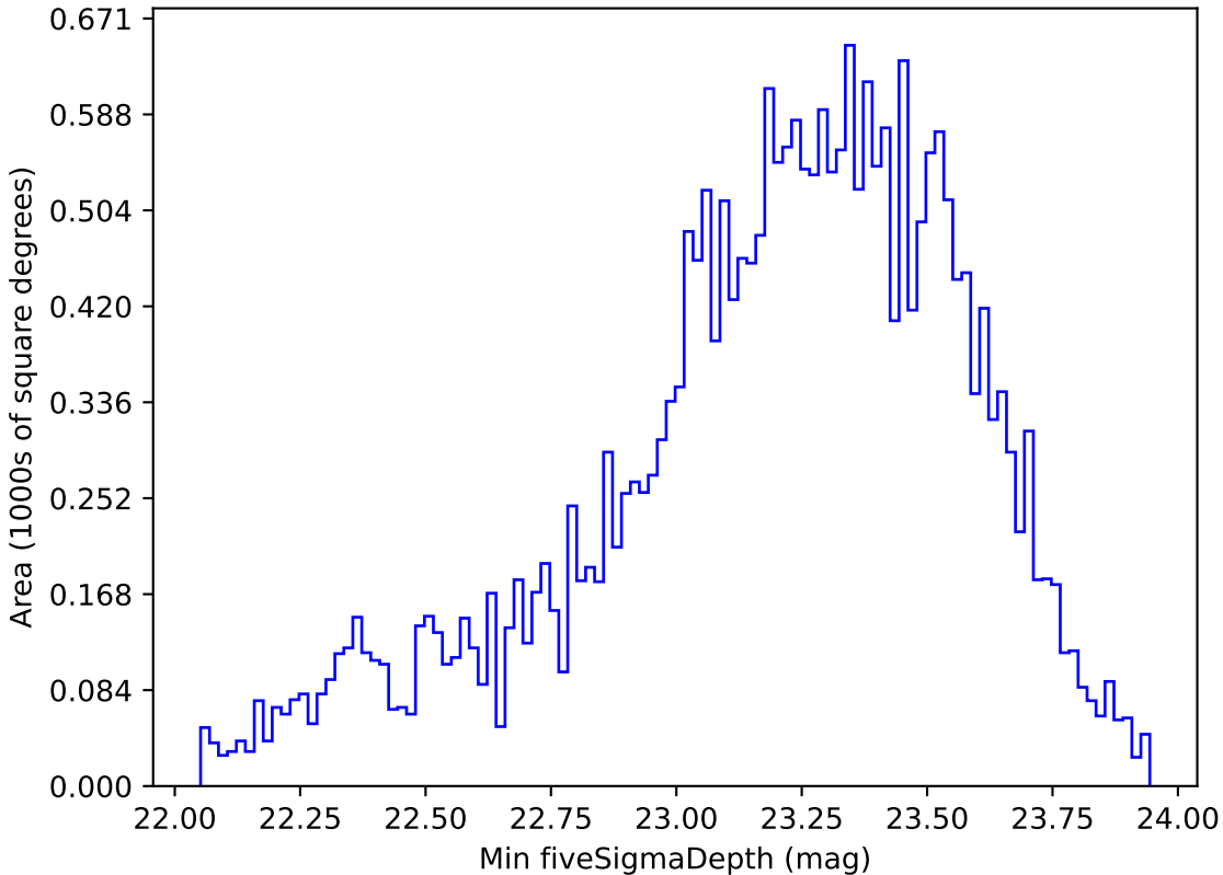
weather_cloudso6v3.4_10yrs All sky g band: Min fiveSigmaDepth
