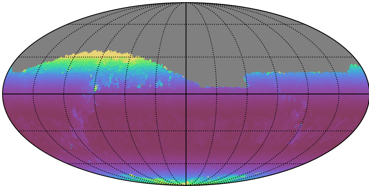
weather_cloudso6v3.4_10yrs Yr 1 z band: Min airmass
