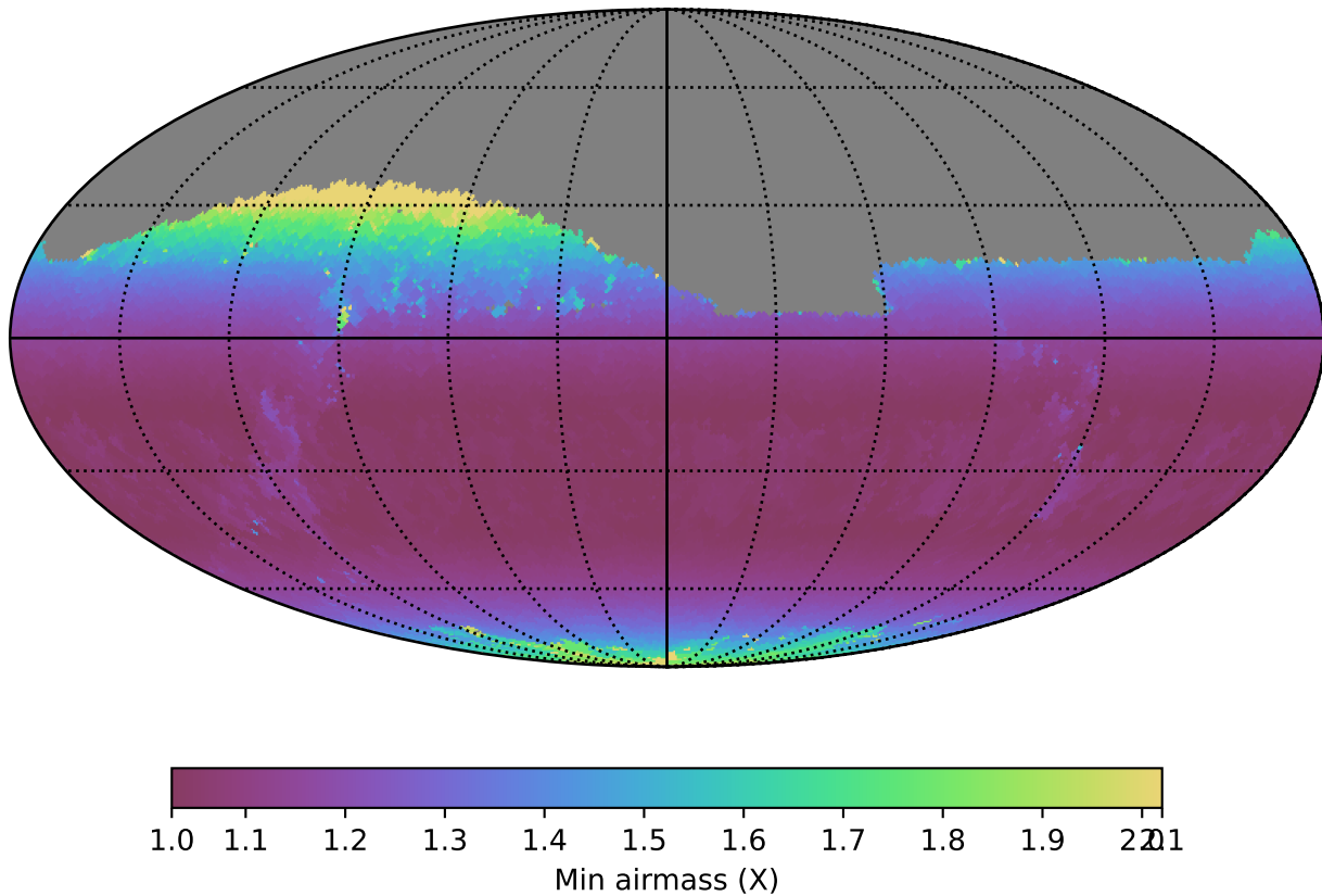
weather_cloudso6v3.4_10yrs Yr 1 z band: Min airmass
