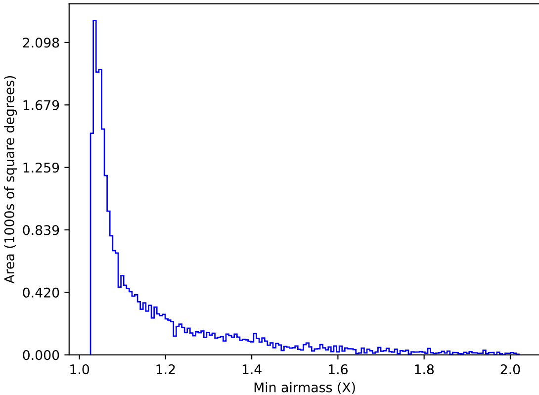
weather_cloudso6v3.4_10yrs Yr 1 z band: Min airmass
