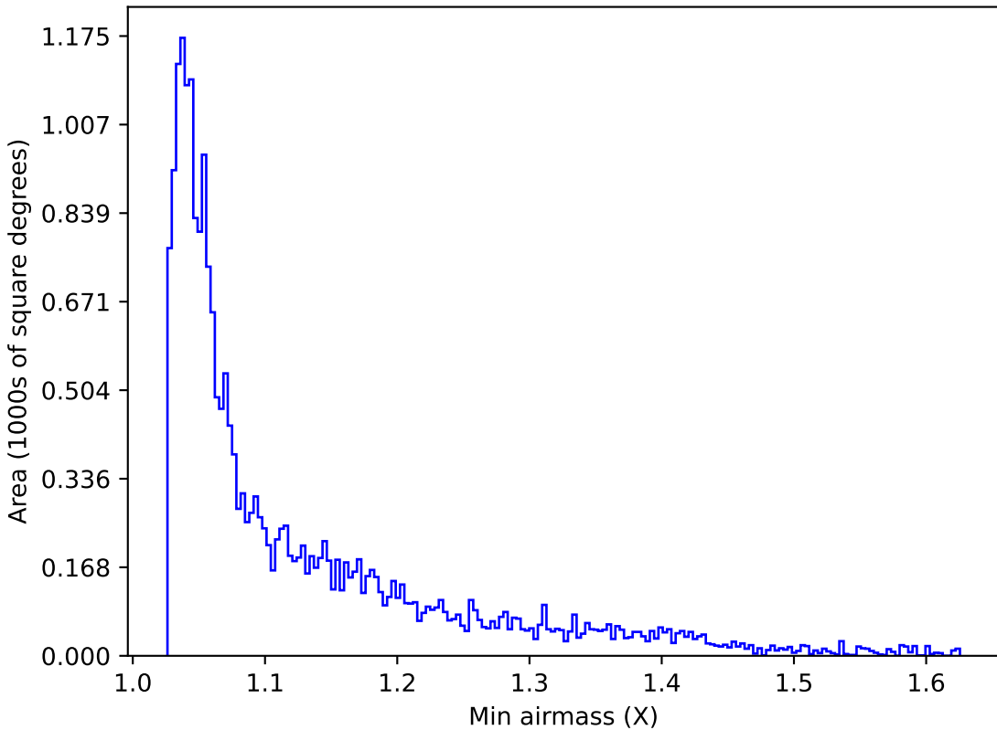
weather_cloudso6v3.4_10yrs Yr 1 y band: Min airmass
