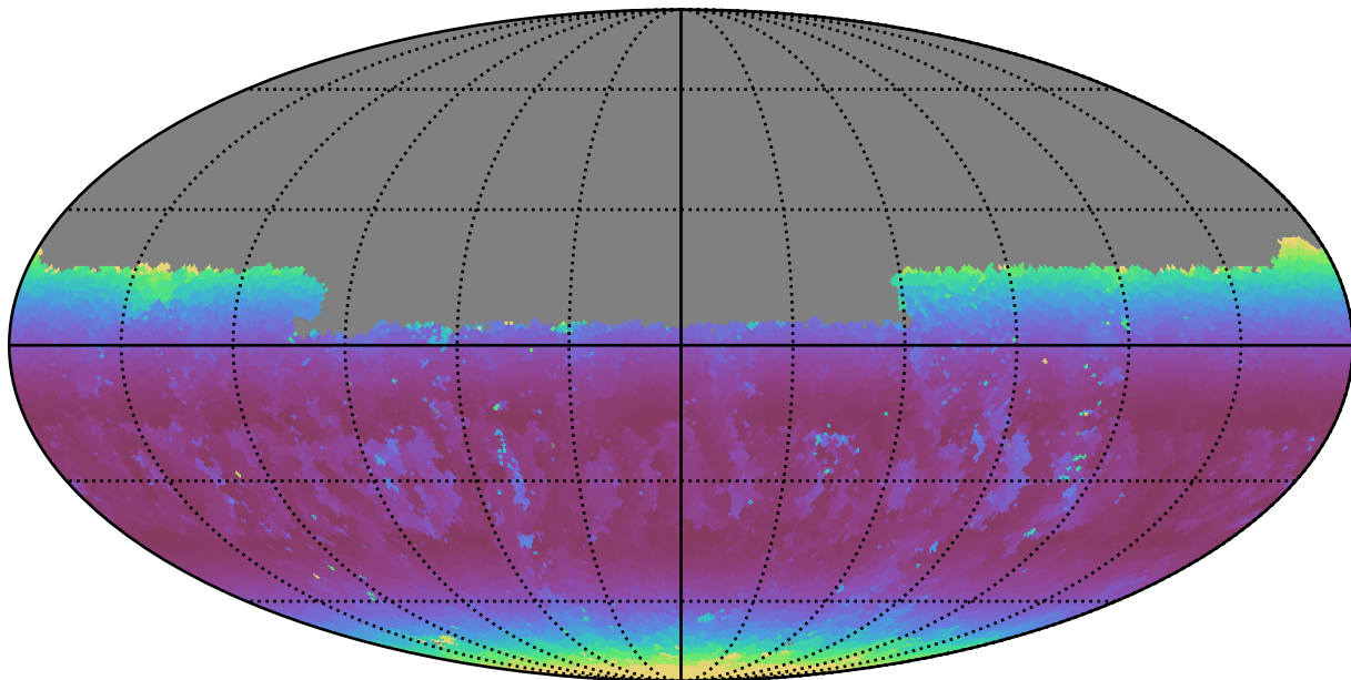
weather_cloudso6v3.4_10yrs Yr 1 u band: Min airmass
