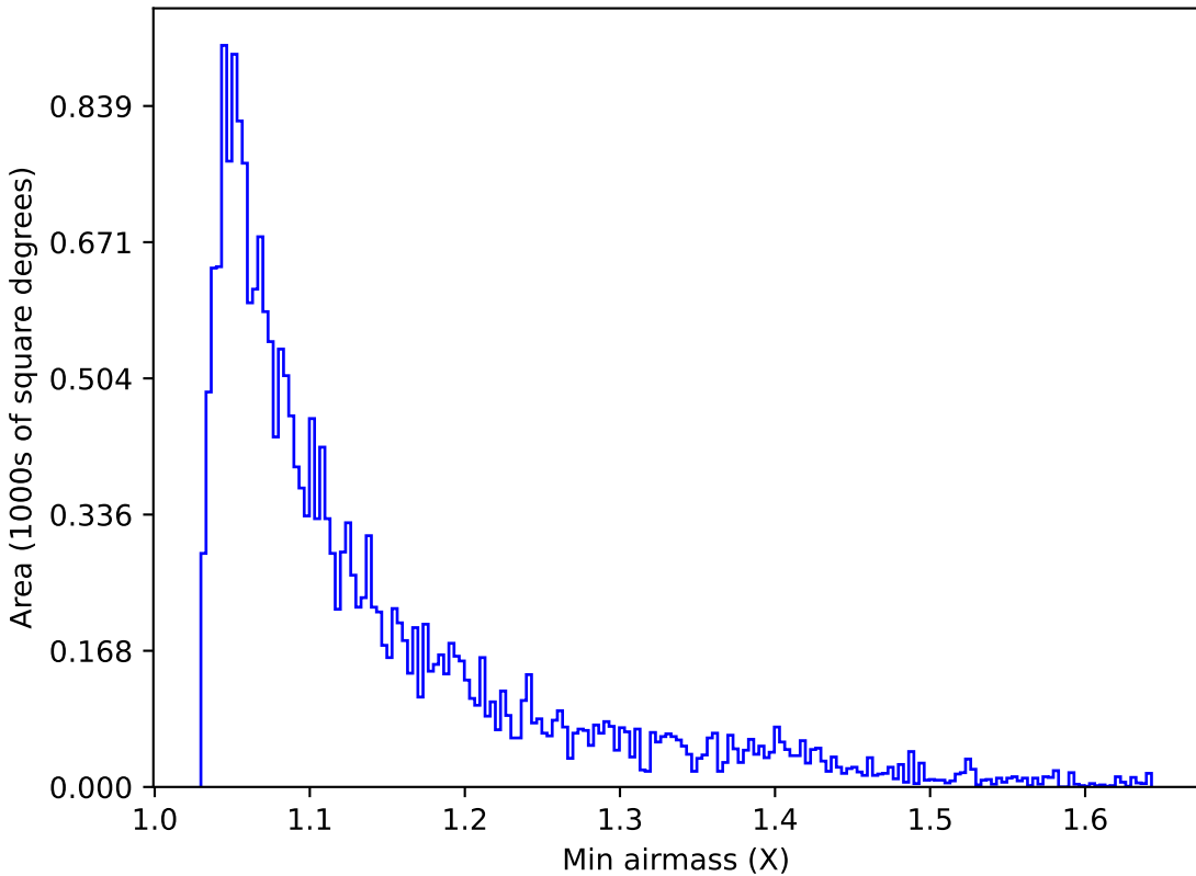
weather_cloudso6v3.4_10yrs Yr 1 u band: Min airmass
