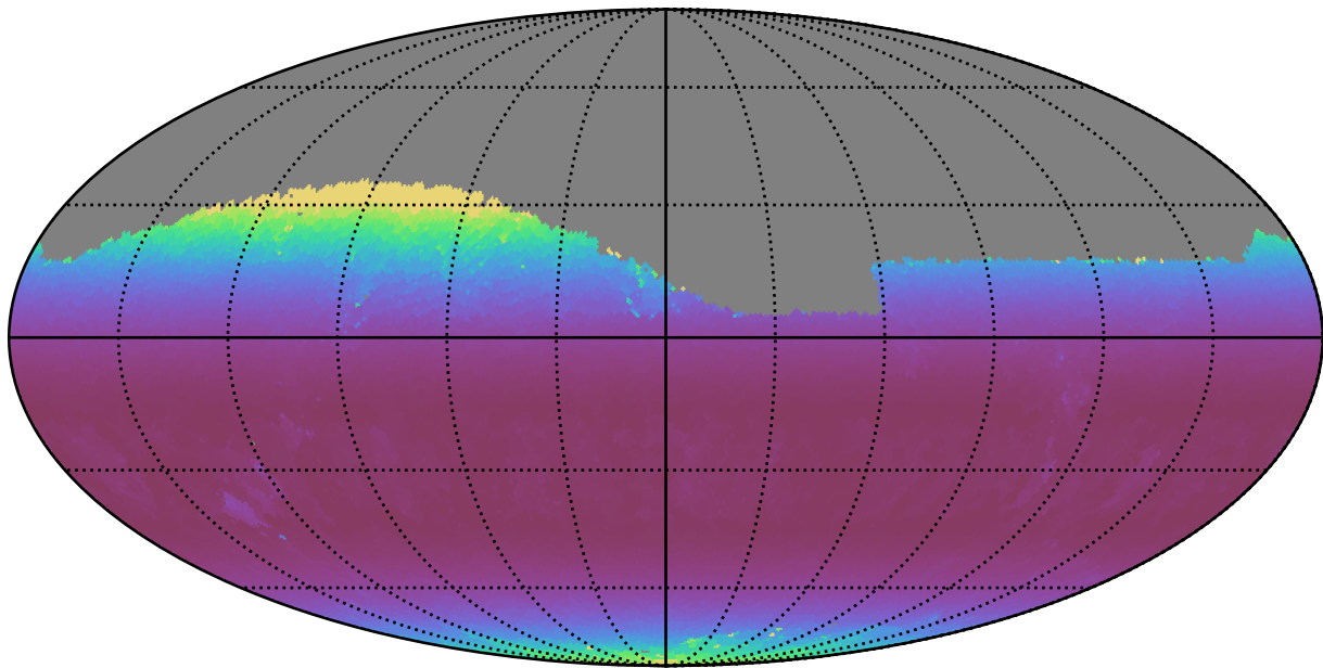
weather_cloudso6v3.4_10yrs Yr 1 r band: Min airmass
