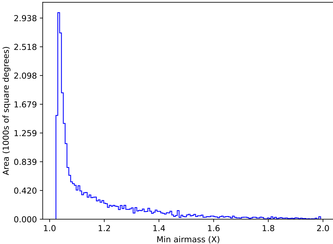
weather_cloudso6v3.4_10yrs Yr 1 r band: Min airmass
