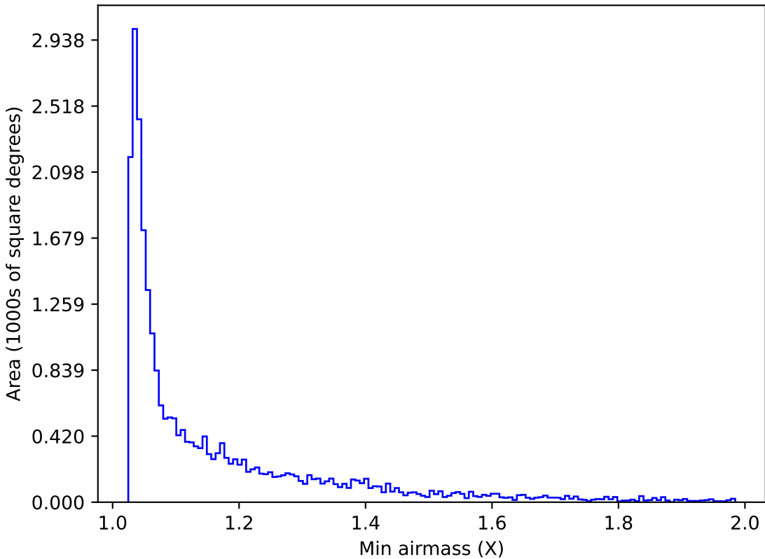
weather_cloudso6v3.4_10yrs Yr 1 i band: Min airmass
