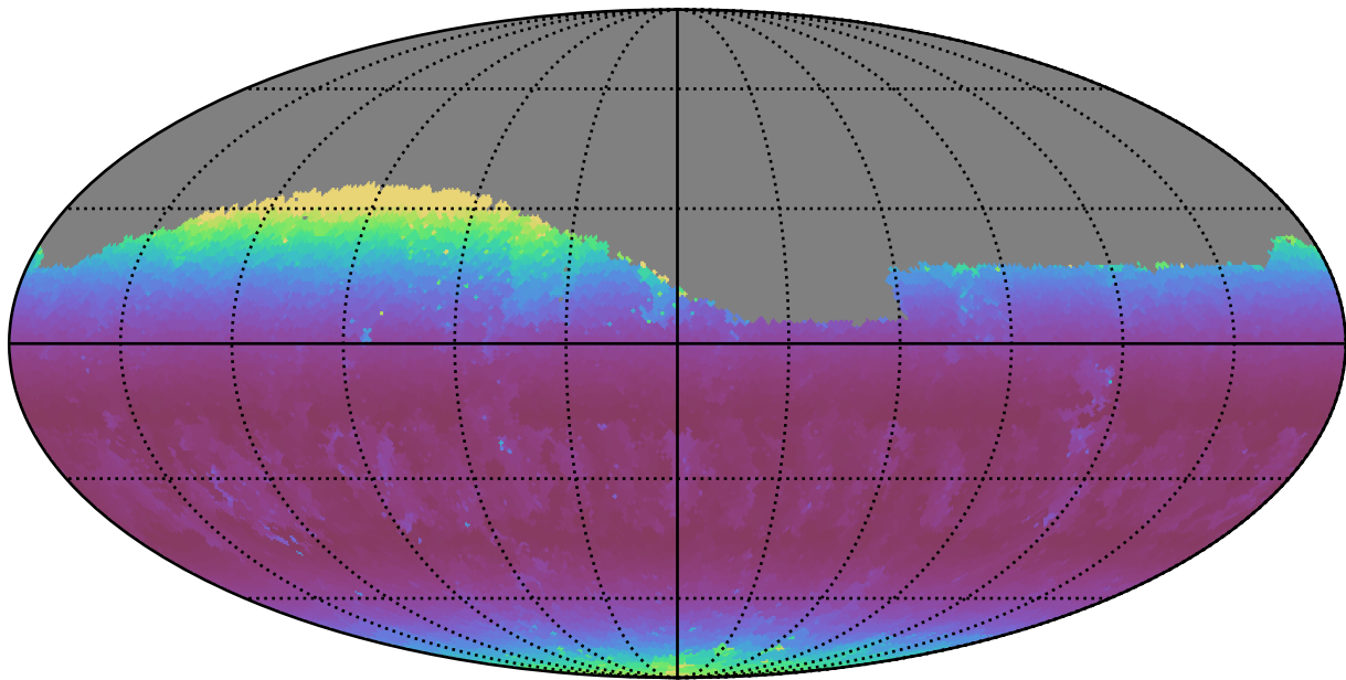
weather_cloudso6v3.4_10yrs Yr 1 g band: Min airmass
