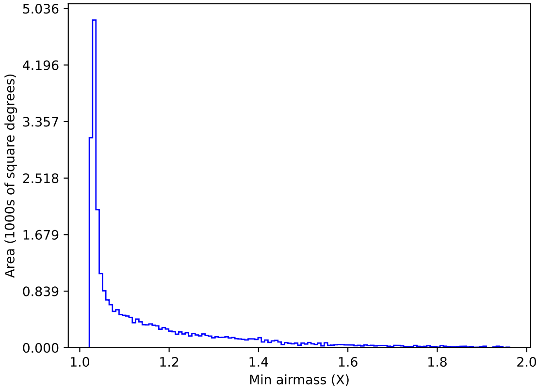
weather_cloudso6v3.4_10yrs Yr 1 all bands: Min airmass
