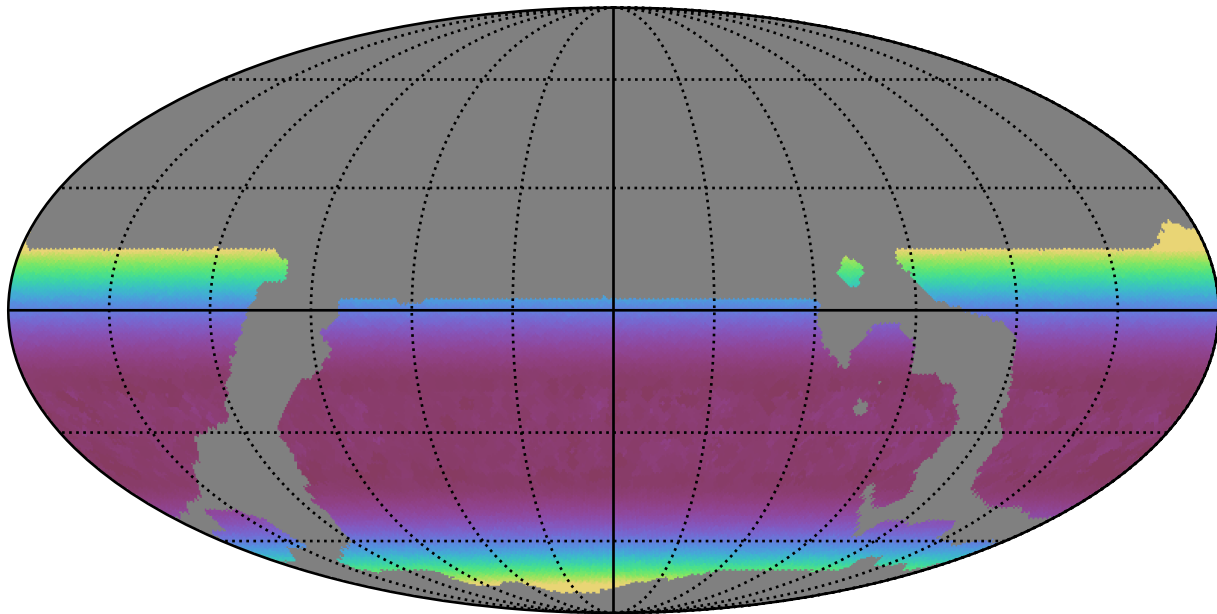
weather_cloudso6v3.4_10yrs WFD z band: Min airmass
