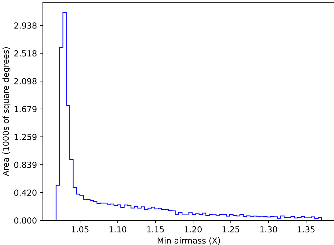
weather_cloudso6v3.4_10yrs WFD z band: Min airmass
