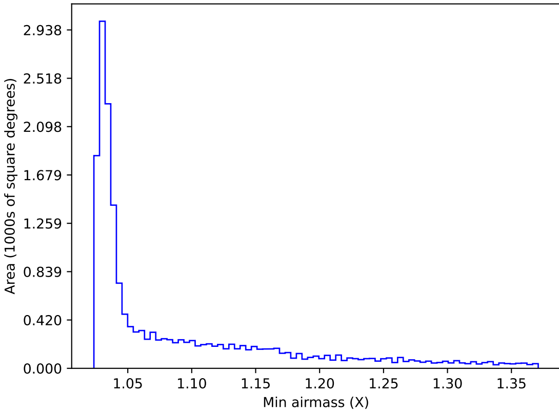
weather_cloudso6v3.4_10yrs WFD y band: Min airmass
