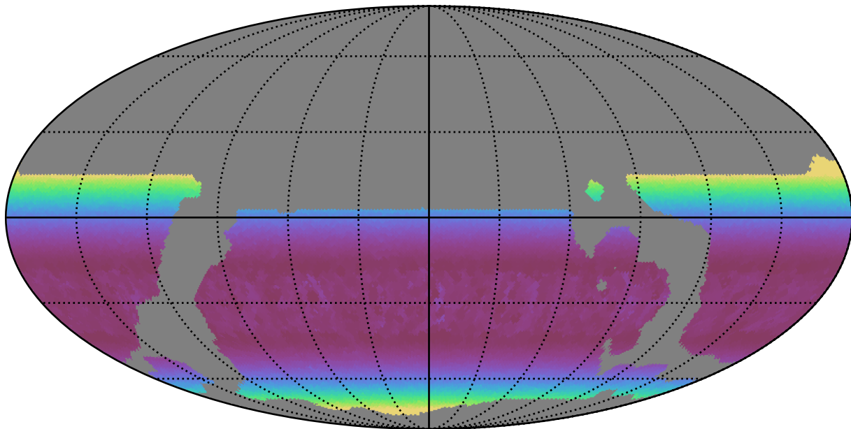
weather_cloudso6v3.4_10yrs WFD u band: Min airmass
