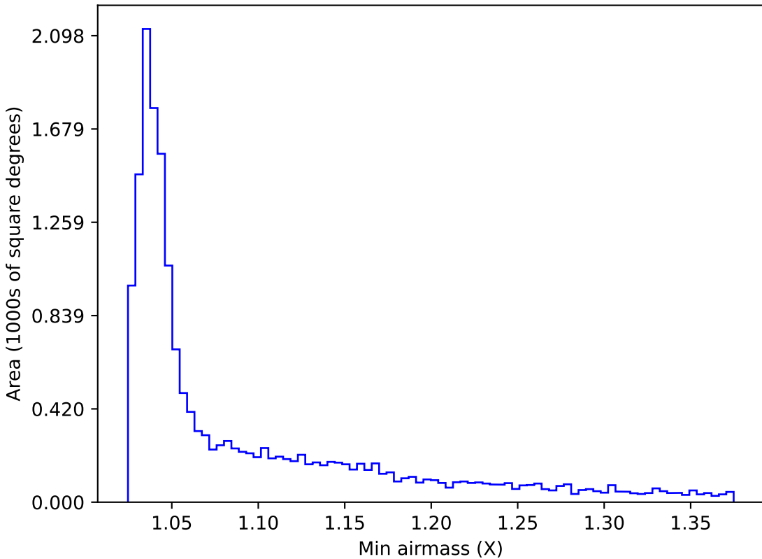
weather_cloudso6v3.4_10yrs WFD u band: Min airmass
