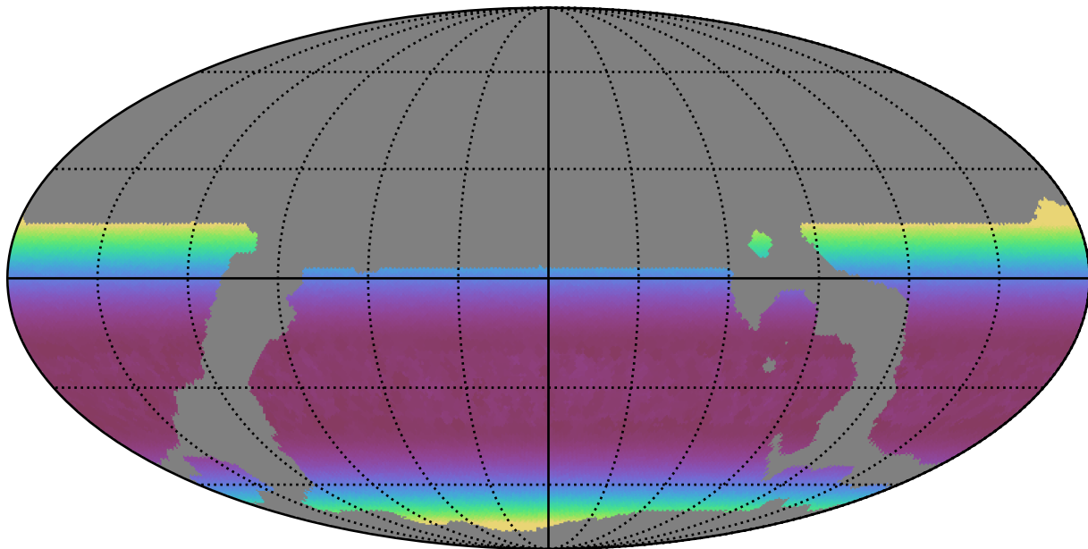
weather_cloudso6v3.4_10yrs WFD r band: Min airmass
