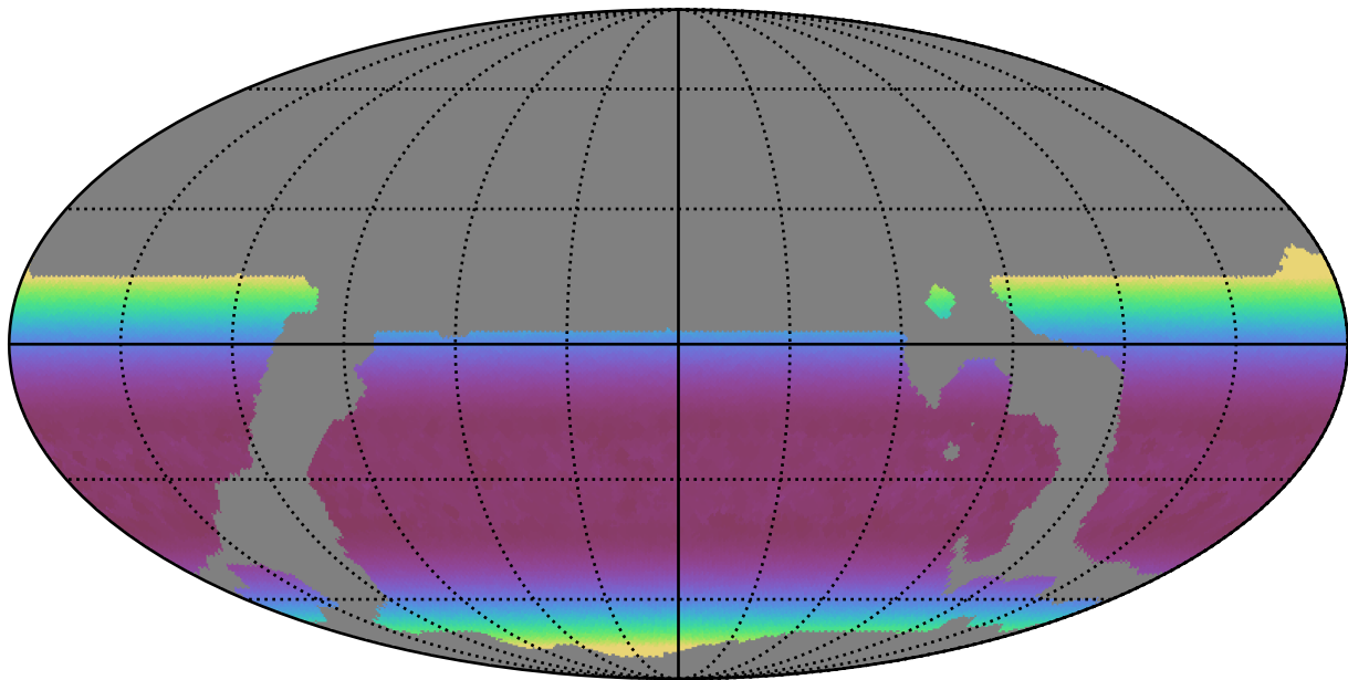
weather_cloudso6v3.4_10yrs WFD i band: Min airmass
